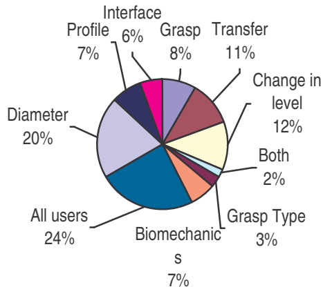
Figure 6 All variables
